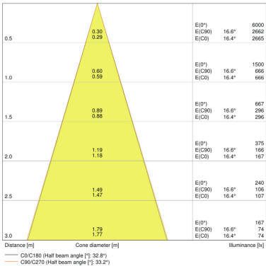
SPOT FIX DIM 8 W 4000 K IP44 SI
